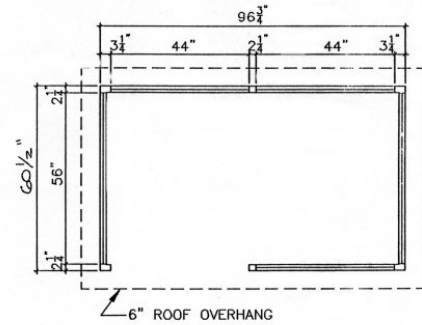
6'x 8' FLOOR PLAN
