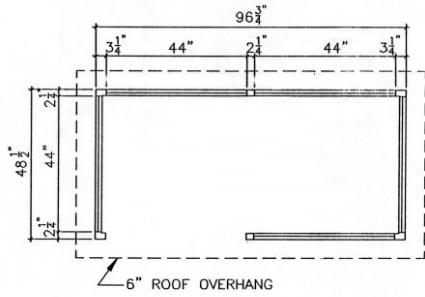
4'x 8' FLOOR PLAN
