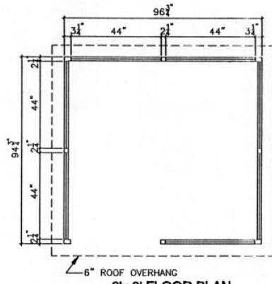
8'x 8' FLOOR PLAN
