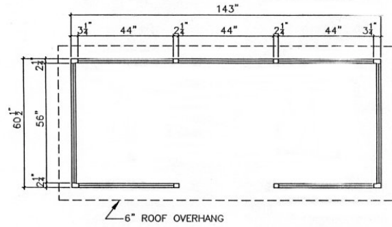
5'x 12' FLOOR PLAN
