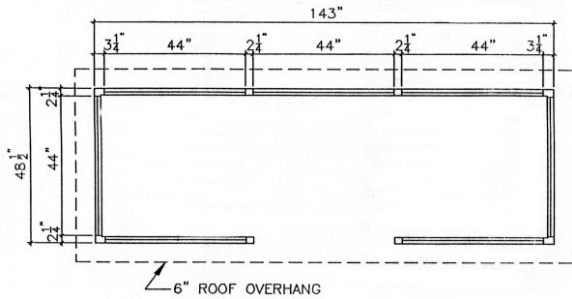
4'x 12' FLOOR PLAN
