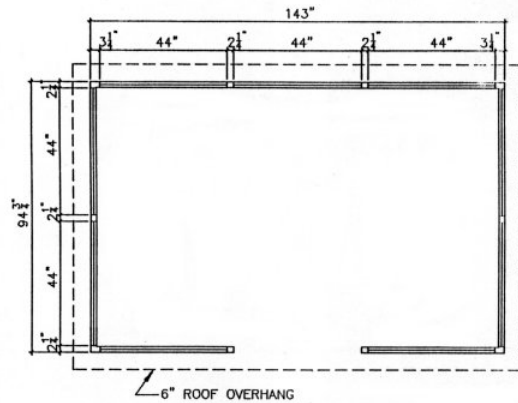
8'x 12' FLOOR PLAN
